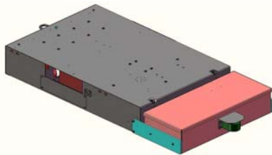
FIGURE ABOVE Solid View of TUNNEL AGC with Electrically Actuated Tow Pin and Proximity Switch in Rear of TUNNEL AGC
